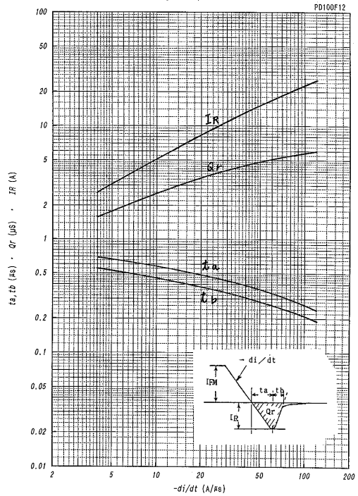
逆回復特性(代表例) REVERSE RECOVERY CHARACTERISTICS (TYP) Tj=150°C, IFR=100 A
